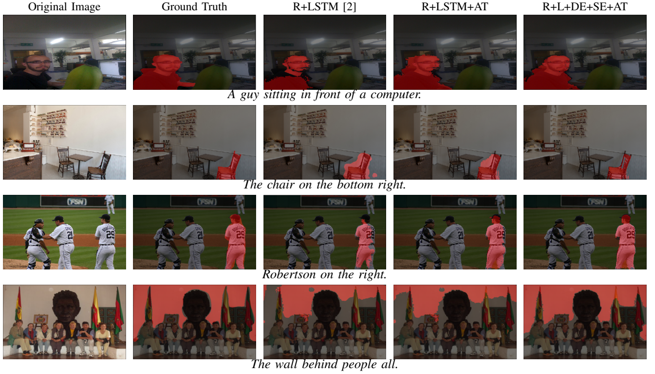
Fig. 4: Visualization results of referring image segmentation. We compare our two proposed models with baseline R+LSTM [2]. The fourth and fifth column are our proposed approaches.
