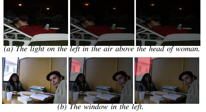
Fig. 8: Failure cases of our model. Given the input images (left) and corresponding referring expressions (below), the predicted referred regions by our model (right) and the ground truth segment masks (middle) are shown.
