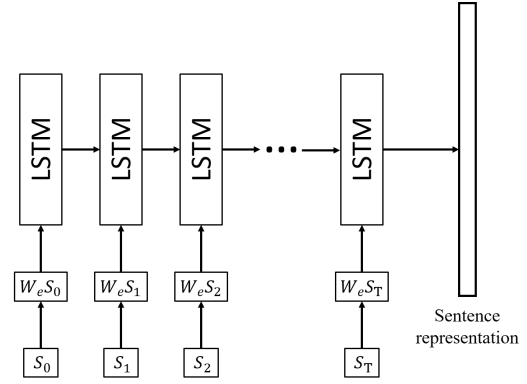
Fig. 3: The structure of the LSTM-based language encoder. This model takes the embedded word after a word embedding matrix as input at each time step.
