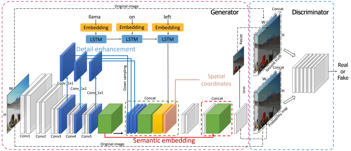
Fig. 2: Network architecture of the proposed ASGN model. It mainly consists of two parts: the generator (left) and the discriminator (right). The generator employs the fully convolutional networks as the backbone to extract image features. We extract feature maps from the network backbone (conv3, conv4 and conv5) as the multi-scale features (blue connection) to enhance the details and then concatenate them with image feature (green block), language feature from LSTM (yellow block) and spatial coordinates (orange block). Then, the fused features are fed into the following two convolutional layers. The semantic features (red connection) are concatenated to the final features before the mask prediction to reduce the ambiguity introduced by word embedding. After generating predictions, a discriminator is introduced to relieve the distribution inconsistencies. In the discriminator network, we first re-size the predictions to the same size as the original images and then concatenate the original image with the predicted masks and real masks respectively. After that, these two image stacks are fed into a classification network with six layers.
