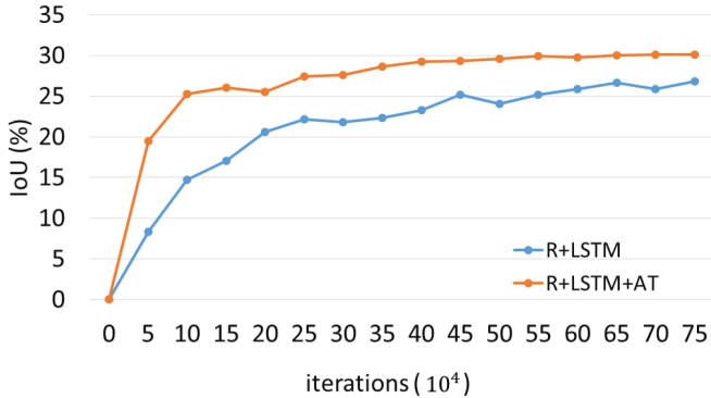
Fig. 7: IoU across training iterations on the UNC dataset on validation data with and without adversarial training.
